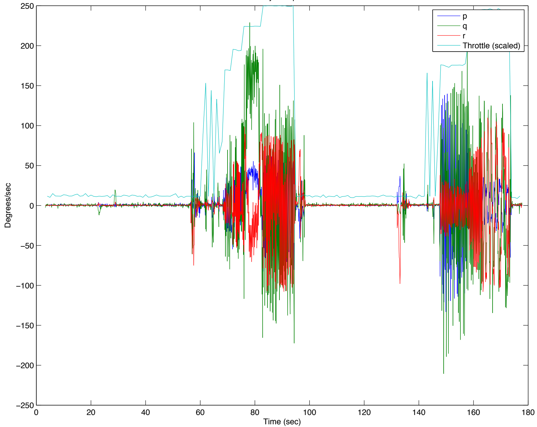
Gyroscope
