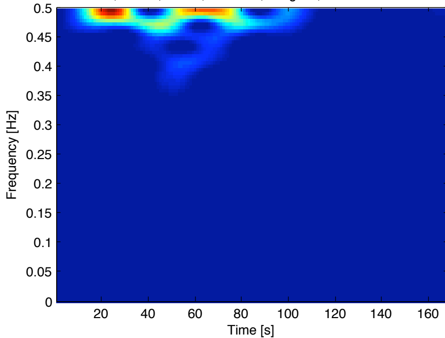
SP, Lh=21, Nf=84, lin. scale, imagesc, Threshold=5%
